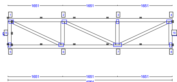
1 | GNA20 1015 105 x 142 | M 1:5
